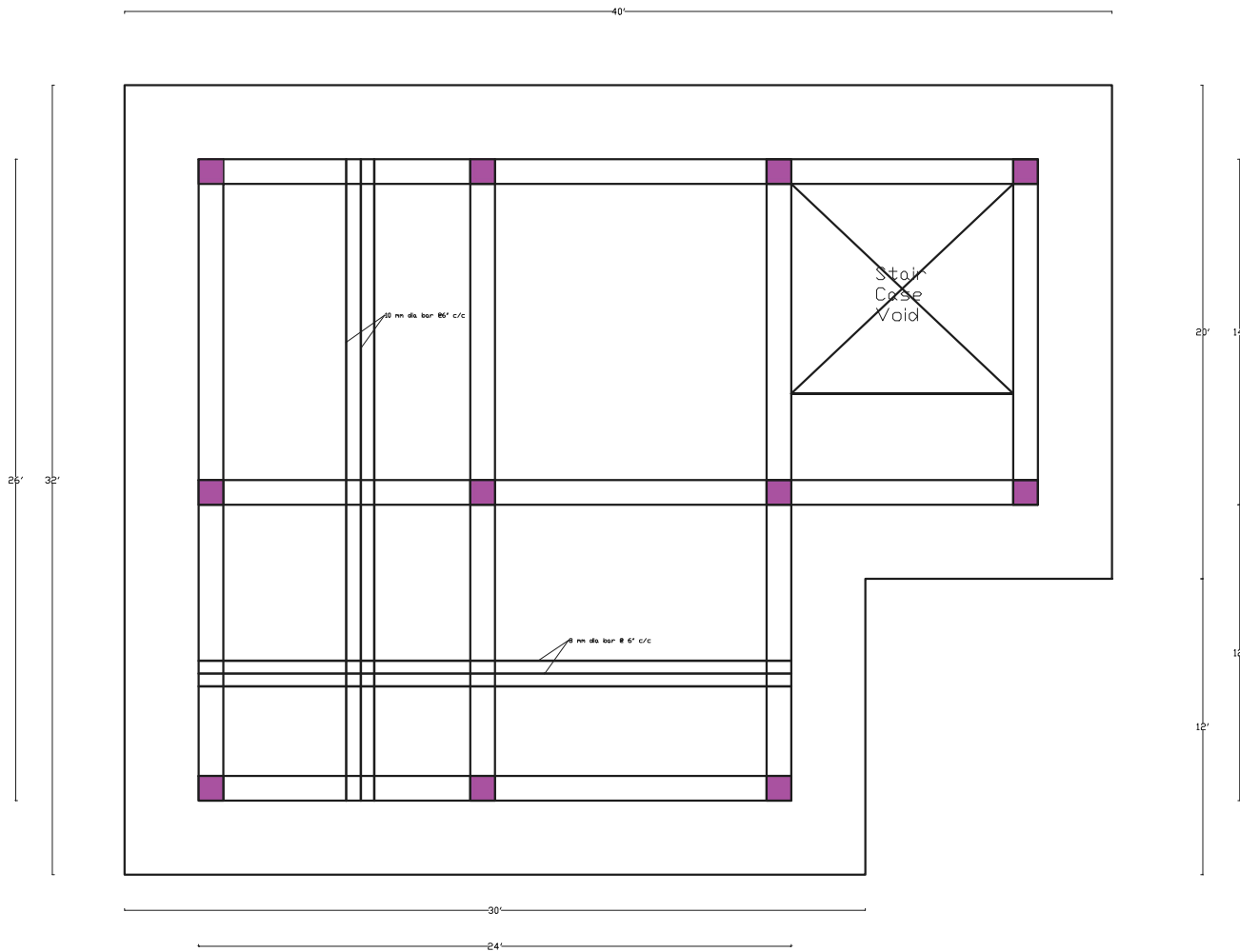
First Floor Bottom Reinforcement
