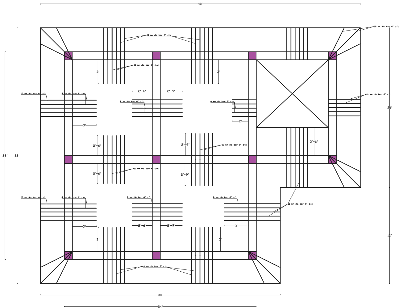
First Floor Top Reinforcement
